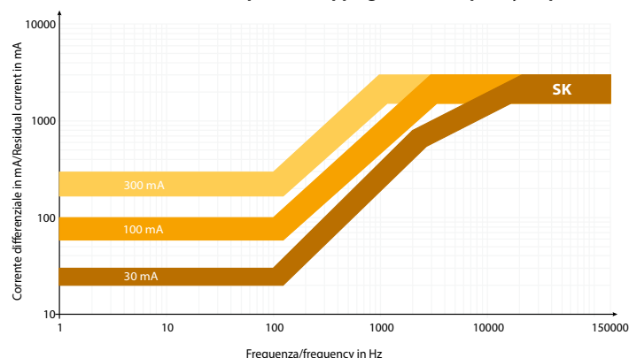
Curva di intervento in frequenza / Tripping current frequency response
