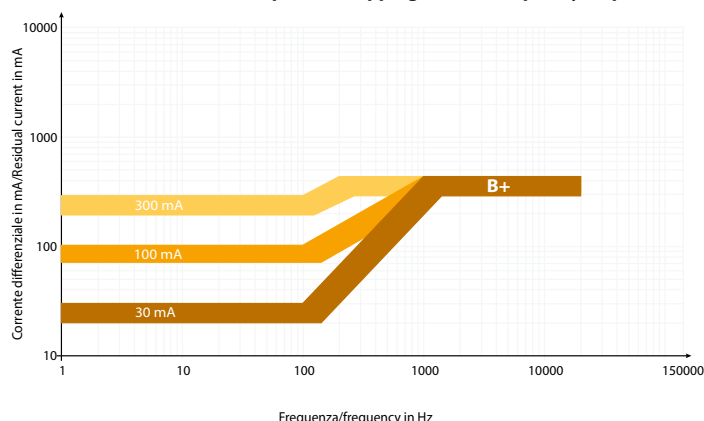
Curva di intervento in frequenza / Tripping current frequency response
